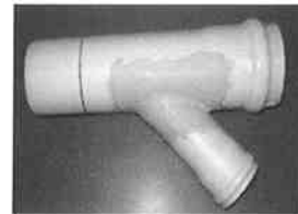
Sample Code Z1504H.150.100 Junct 150Ø 100Ø Sewer RRJ SN16
