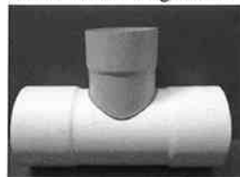
Sample Code 704.375.100.45U Junction 375Ø 100Ø Stormwater Unglassed
